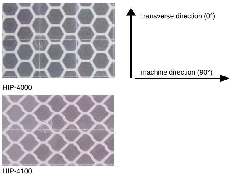
Figure 1 - Sealing pattern and application directions
